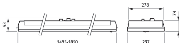
RC460B G2 LED34S/840 PSD W30LEXT VPC W
