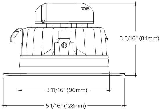
COREPRO DOWNLIGHT 4"
