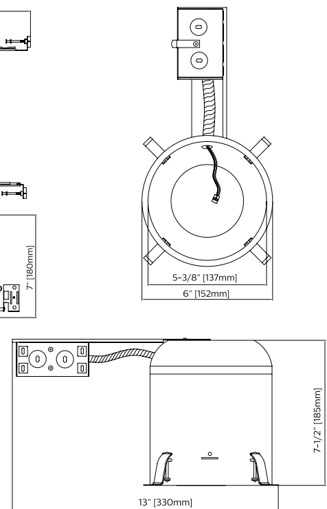
CP5RR: 5" IC/Airseal Remodeler Housing
