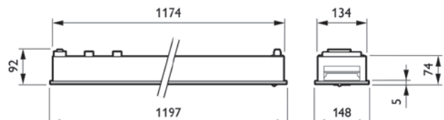
RC415B G2 LED20S/840 PSD W15L120 VPC W
