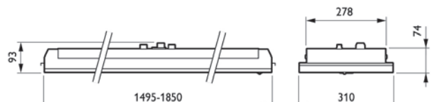
RC462B G2 LED34S/840 PSD W31LEXT VPC W
