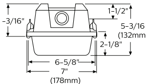
Shallow acrylic (A) and polycarbonate (P) lens
