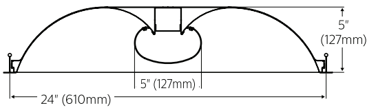
HP90_LED_2x4
