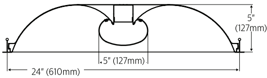
HP90_LED_2x4
