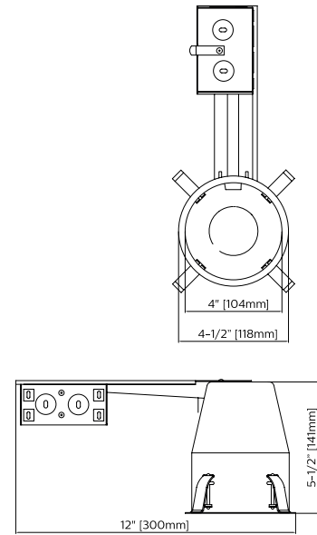
CP4RR: 4" IC/Airseal Remodeler Housing
