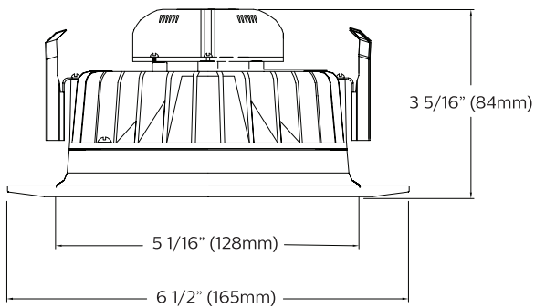
COREPRO DOWNLIGHT 5"
