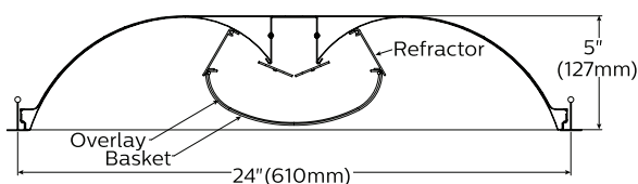
Coffaire_LED_2x4
